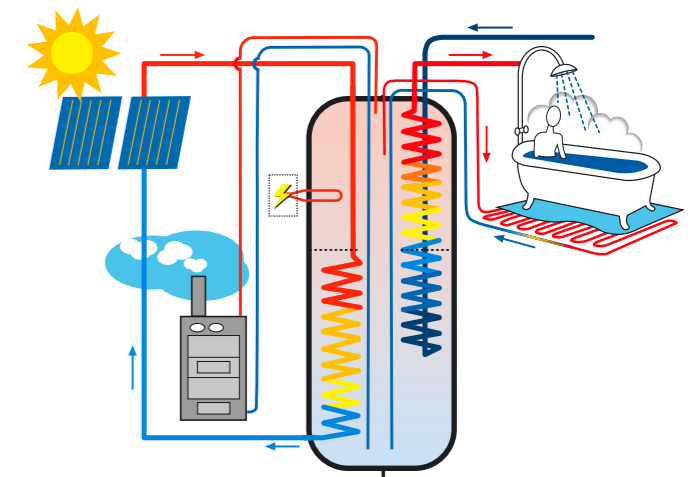
Energy for the tank is brought from the sun, a boiler if required, or other heat source.
