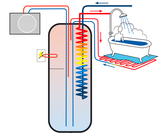
Connection of air/water heat pump.
