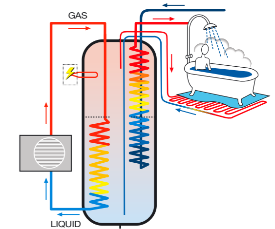
Energy transfer to the accumulator tank through the hot gas coil.
